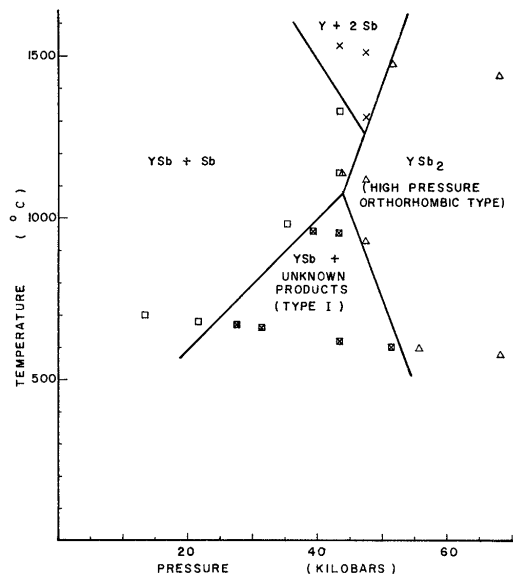
Figure 6.—Y-2Sb reaction product diagram.
