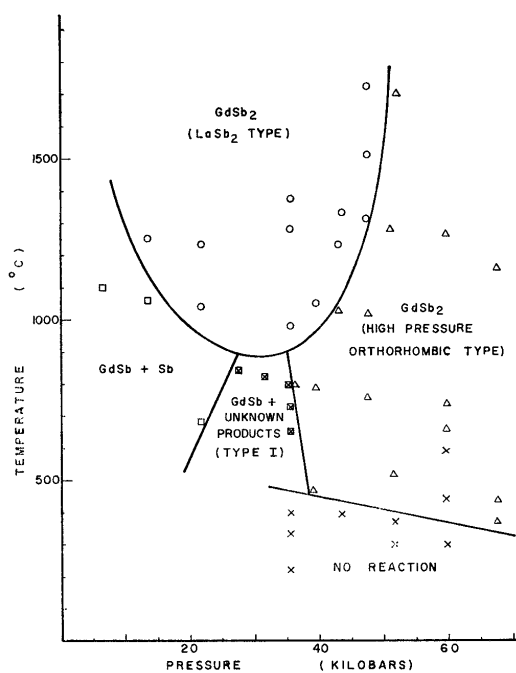
Figure 2.—Gd-2Sb reaction product diagram.
