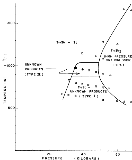
Figure 8.—Tm-2Sb reaction product diagram.
