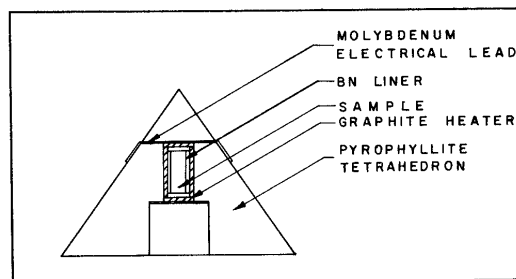
Figure 1.—Cross section of tetrahedral sample geometry.
