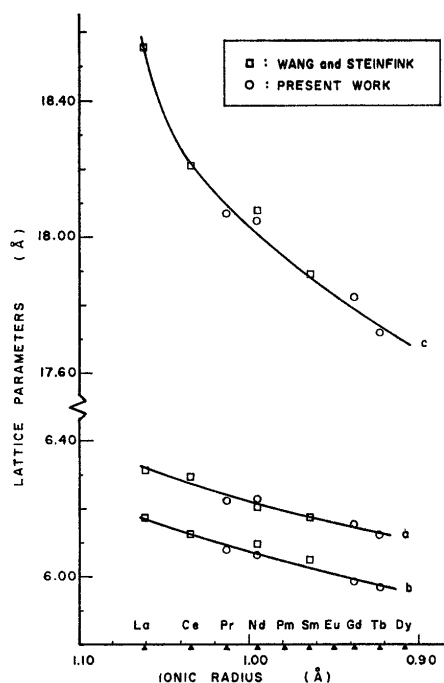
Figure 12.—Variation of lattice parameters with the ionic radius of LaSb 2 -type rare earth diantimonides.
