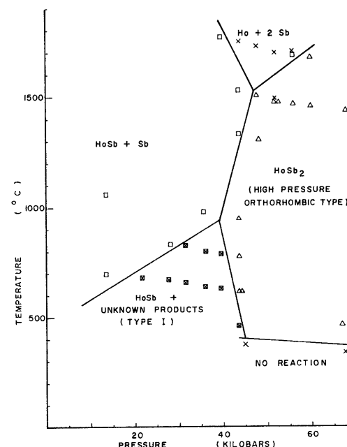
Figure 5.—Ho-2Sb reaction product diagram.
