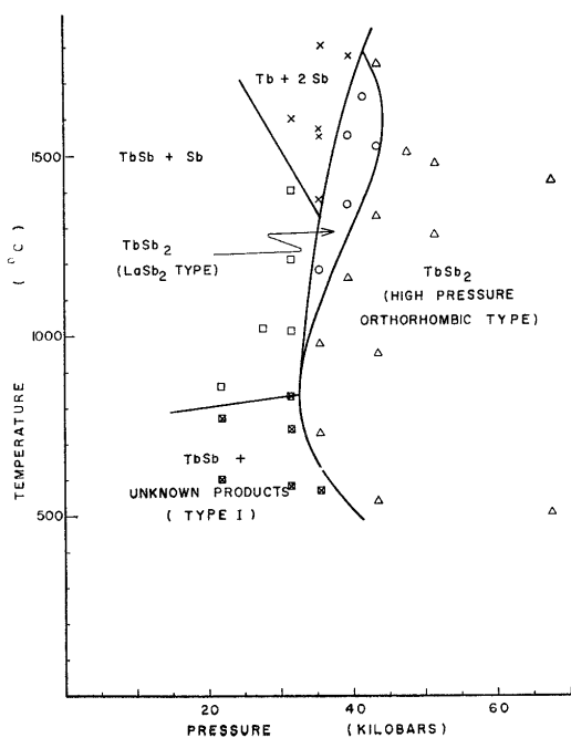
Figure 3.—Tb-2Sb reaction product diagram.
