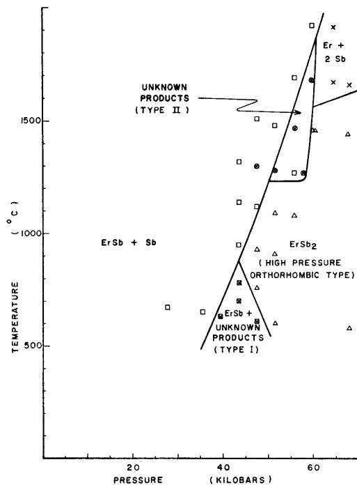
Figure 7.—Er-2Sb reaction product diagram.
